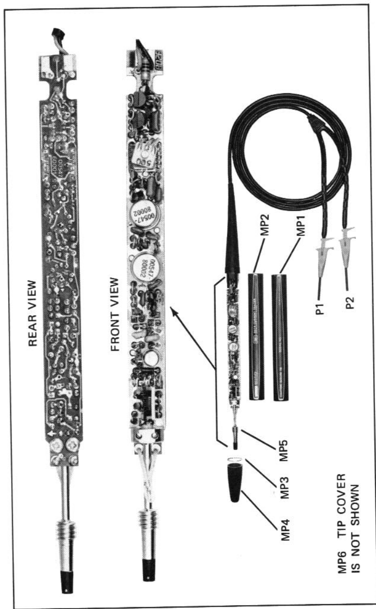
Figure 6. Exploded View of Current Tracer
