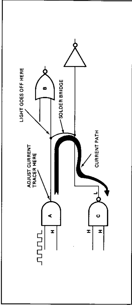
Figure 4. Solder-Bridge in Printed-Circuit
